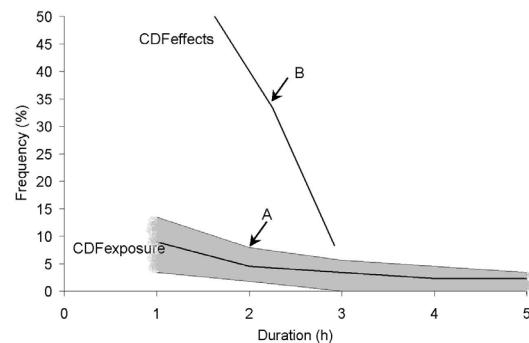
Figure 4. Concentration-Duration-Frequency (CDF) exposure and effect curves ( CDF_{exposure} also has an 90%-uncertainty band)
