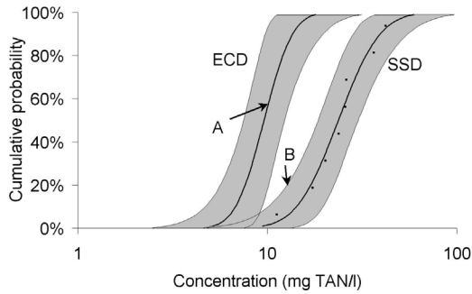
Figure 3. The Exposure Concentration Distribution (ECD) and the salmonid Species Sensitivity Distribution (SSD) of Total Ammonia Nitrogen (TAN) downstream of the wastewater treatment plant of Hove
