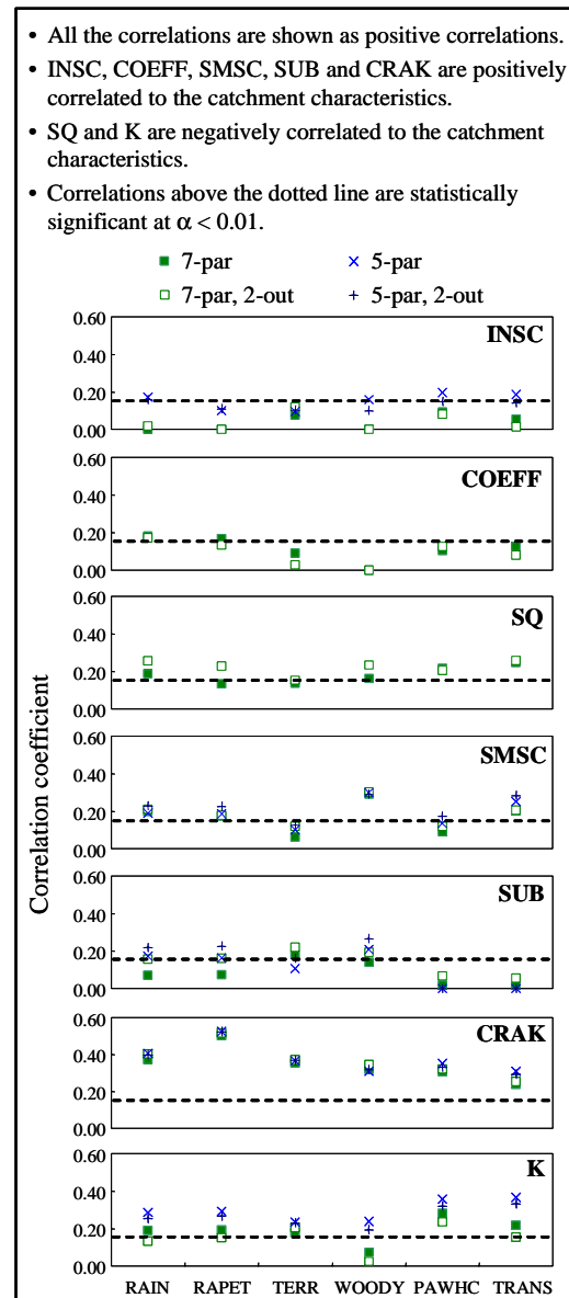
Figure 4. Correlations between optimised SIMHYD parameter values versus various catchment characteristics for the four model types
