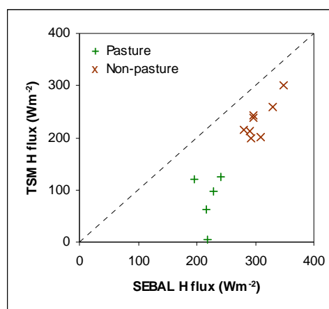
Figure 3. Difference between TSM and SEBAL estimated sensible heat flux at the 13 sites selected for the study.
